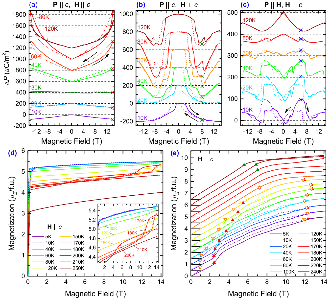
FIG. 6. Magnetic-field dependence of polarization change \Delta P at different temperatures, for (a) \Delta P \parallel c and \mathbf{H} \parallel c axis, (b) \Delta P \parallel c and \mathbf{H} \perp c axis, and (c) \Delta P \parallel \mathbf{H} and \mathbf{H} \perp c axis. In panels (a), (b), and (c), each polarization curve is shifted vertically by 200 \mu\text{C}/\text{m}^2 , 200 \mu\text{C}/\text{m}^2 , and 100 \mu\text{C}/\text{m}^2 , respectively, for the purpose of clarity. \Delta P values marked by cross symbols are plotted in Fig. 7(b) against temperature. (d) Field dependence of the magnetization at various temperatures with magnetic fields applied along the c axis. The inset shows a magnified view of the hysteresis region. (e) Field-dependent magnetization curves at different temperatures when the field is applied perpendicular to c . Each curve is shifted vertically by 0.5 \mu_B/\text{f.u.} for better visibility. Data collected in increasing and decreasing magnetic fields are plotted with solid and dashed lines, respectively. The magnetic phase transitions \mu_0 H_{C1} , \mu_0 H_{C3} , and \mu_0 H_{C4} are indicated by solid up and empty down triangles for the field increasing and decreasing runs, respectively. These phase transitions are determined as local maximum of the \frac{dM}{dH} curves, and are plotted in the \mu_0 H - T phase diagram by symbols of the same colors (Fig. 8). For more details about the determination of the phase boundaries see the Supplemental Material [52].
